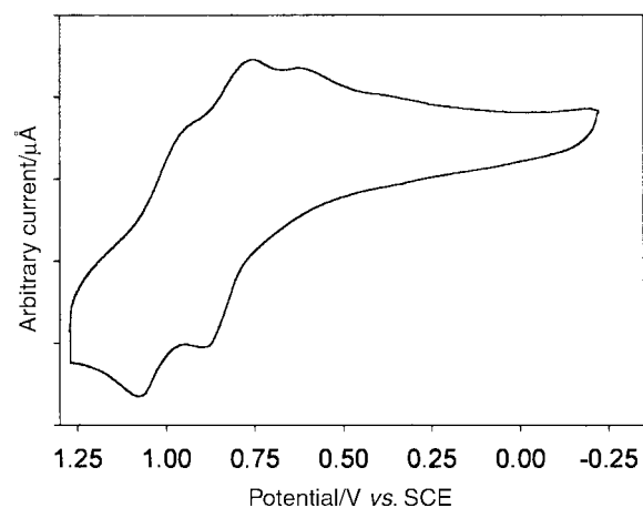
Fig. 2 Cyclic voltammogram of [(Ru(NH_3)_4)(qH_2 \cdot qH_2)]^{4+} in acetonitrile solution (0.15 M TBAPF 6 ). Scan rate 100 mV s -1 .
