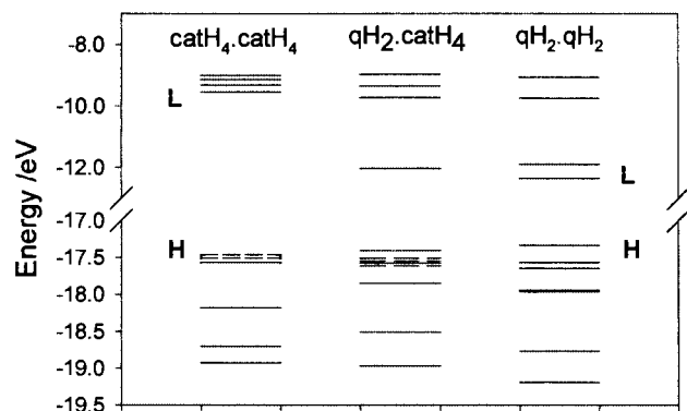
Fig. 9 Relative molecular orbital energies of the symmetric series as labelled. The HOMO is indicated by H and the LUMO by L. The \text{catH}_4 localized Ru d(t_{2g}) orbitals are displayed with hatched lines in the \text{catH}_4\cdot\text{catH}_4 and \text{qH}_2\cdot\text{catH}_4 species.
