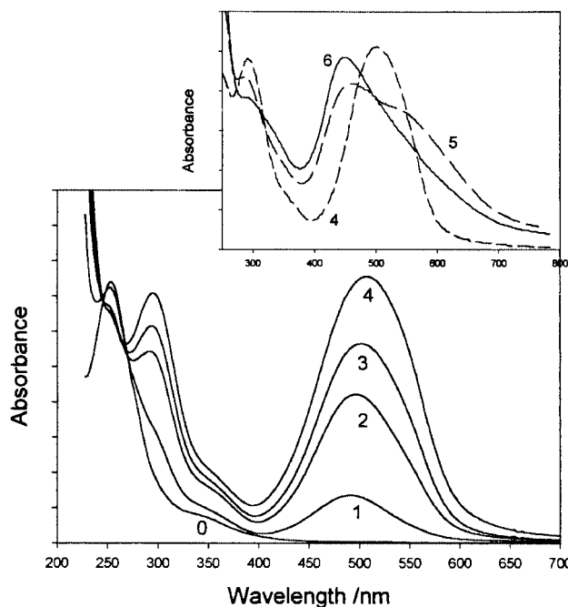
Fig. 3 Ceric titration of a 4.1 \times 10^{-5} \text{ M} solution of [(\text{Ru}(\text{NH}_3)_4)_2(\text{catH}_4\cdot\text{catH}_4)](\text{PF}_6)_4 in 0.1 M \text{H}_3\text{PO}_4 showing the addition of 0–4 equivalents of \text{Ce}(\text{IV}) . Inset; data for 4–6 equivalents of \text{Ce}(\text{IV}) as designated.
