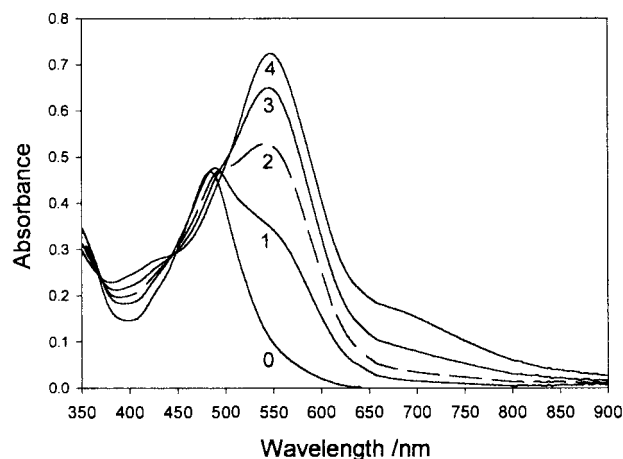
Fig. 4 Ceric titration of a 2.2 \times 10^{-5} \text{ M} solution of [\text{Ru}(\text{bpy})_2(\text{catH}_4\cdot\text{catH}_4)\text{Ru}(\text{NH}_3)_4](\text{PF}_6)_4 in 0.1 M \text{H}_3\text{PO}_4 showing the addition of 0–4 equivalents of \text{Ce}(\text{IV}) .
